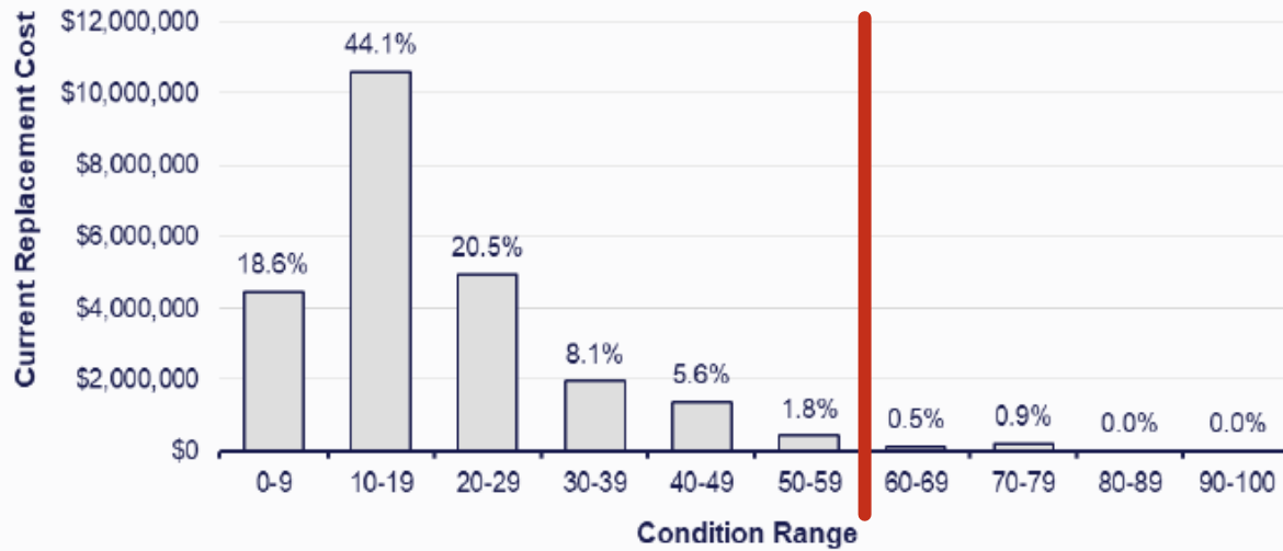
Sealed Road Pavement Condition Profile
