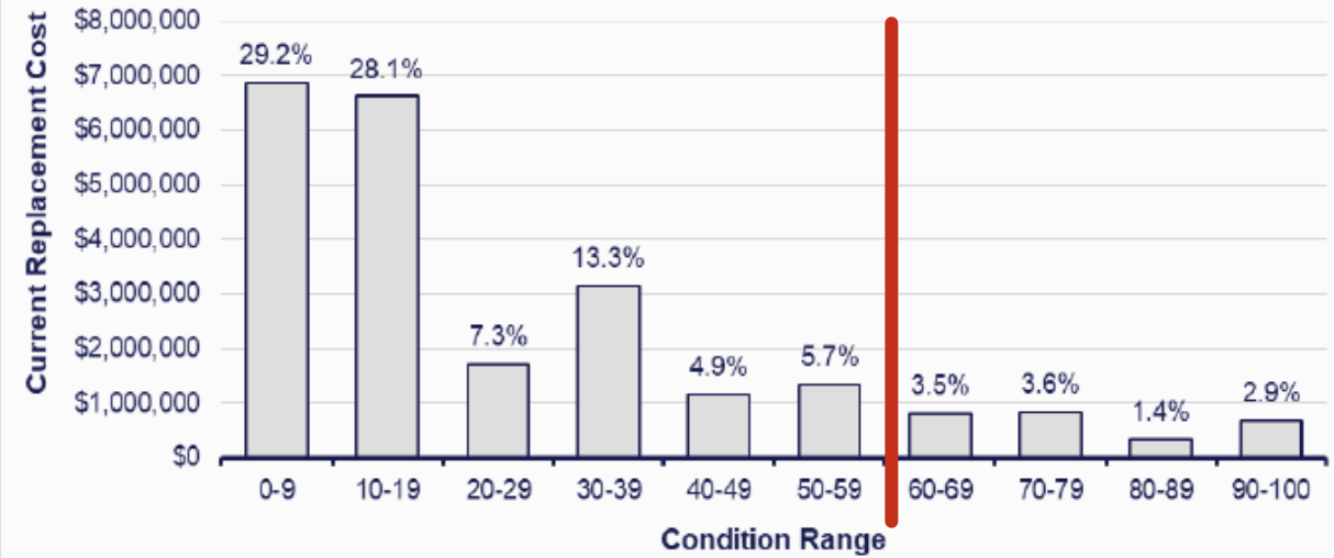
Unsealed Sheeted Road Condition Profile
